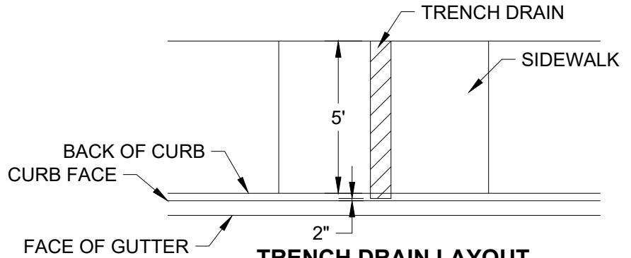
TRENCH DRAIN LAYOUT
