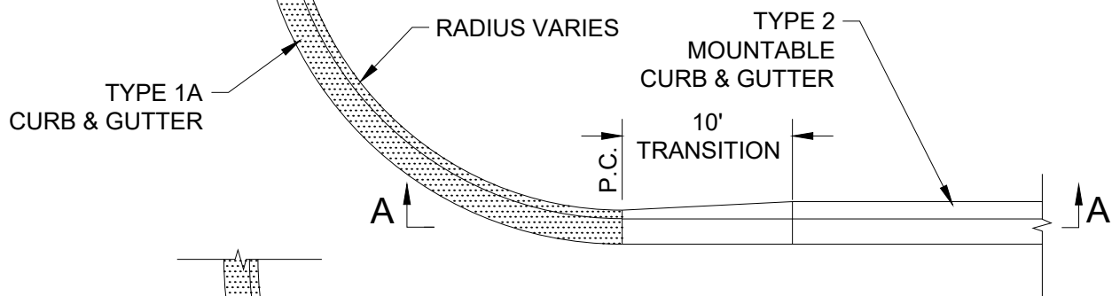
TRANSITION AT RADIUS
