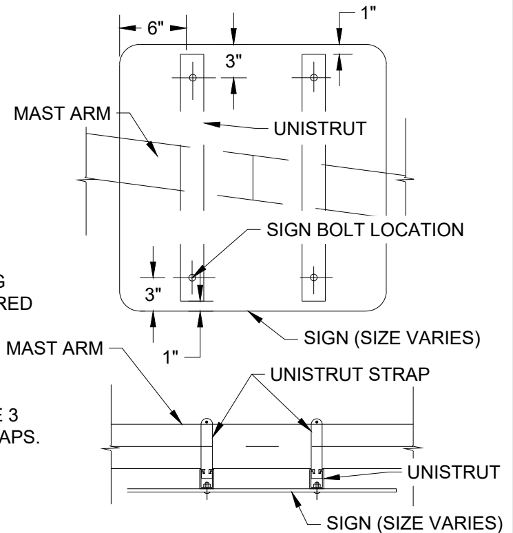
DETAIL "B" GALVANIZED UNISTRUT
