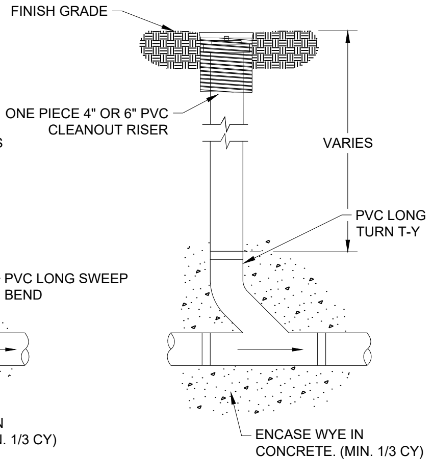
IN-LINE CLEANOUT
