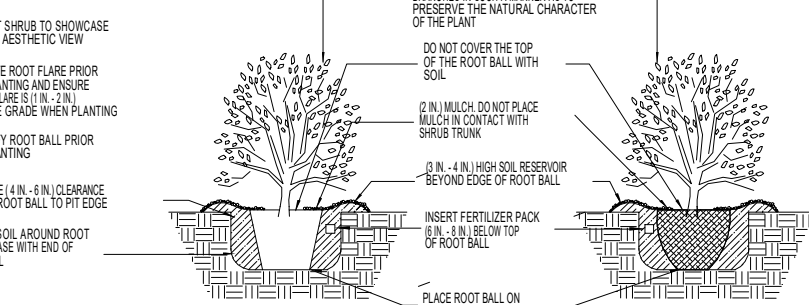
3 SHRUB PLANTING DETAIL
