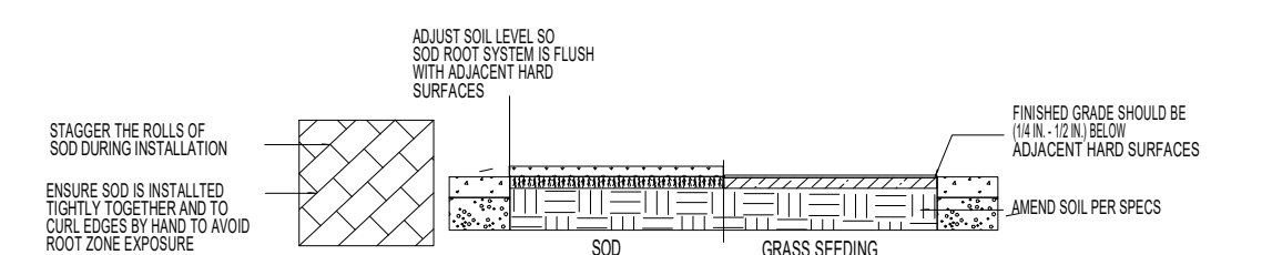
5 TYPICAL TURF INSTALLATION
