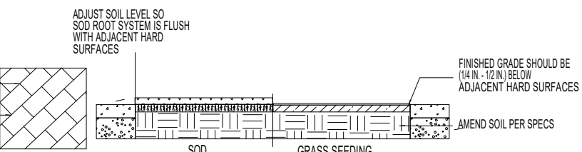
5 TYPICAL TURF INSTALLATION
