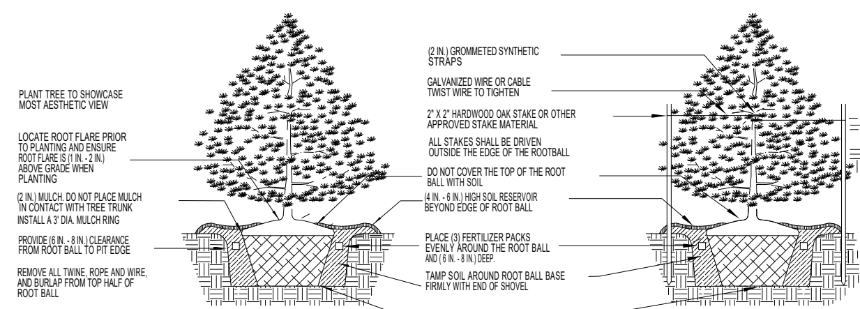
2 CONIFEROUS TREE PLANTING DETAIL
