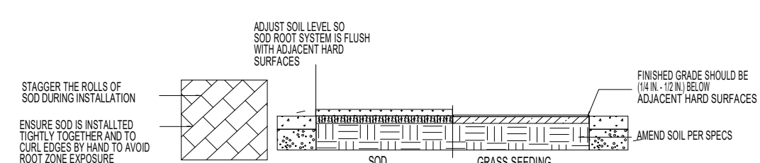
5 TYPICAL TURF INSTALLATION
