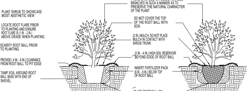
3 SHRUB PLANTING DETAIL TYPICAL INSTALLATION FOR POTTED AND BAR SHRUBS
