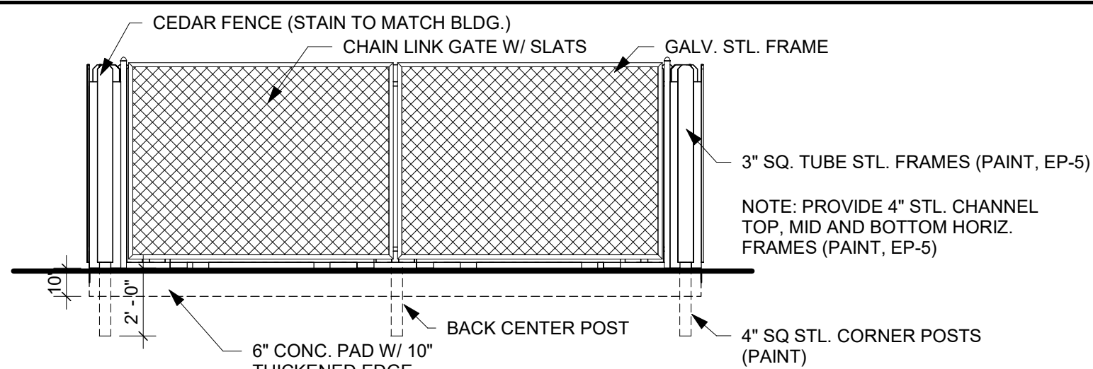
2 DUMPSTER ENCLOSURE A001 1/4" = 1'-0"
