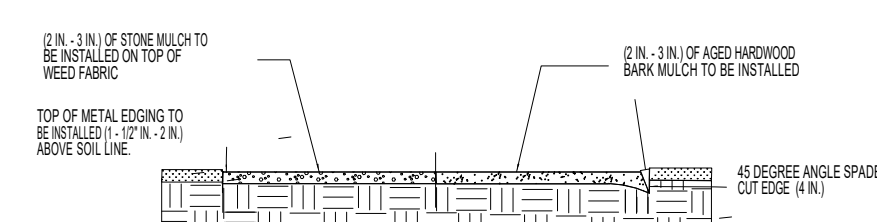
6 TYPICAL MULCH INSTALLATION
