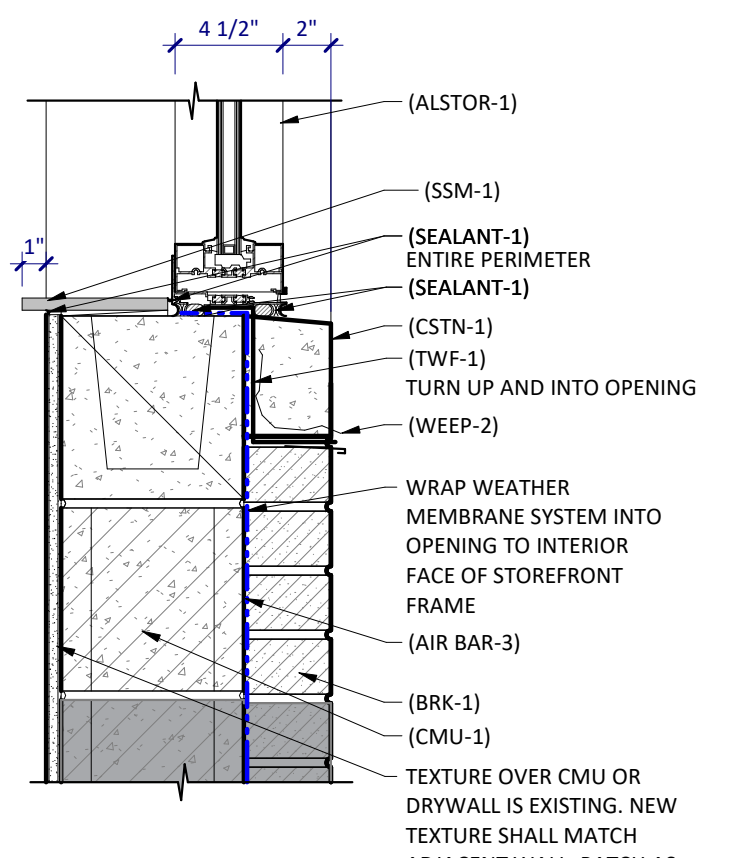
5A A311 NEW BRICK SILL DETAIL SCALE: 1 1/2" = 1'-0"
