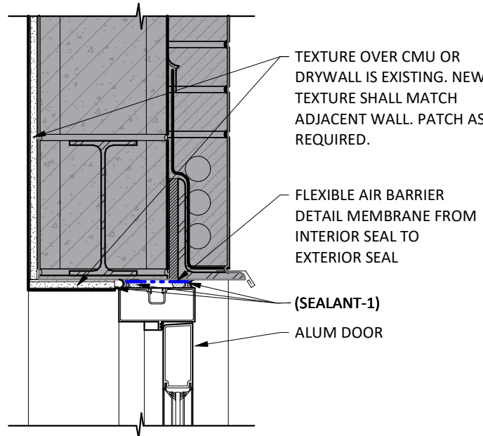
6B A311 ALUM HEAD DETAIL SCALE: 1 1/2" = 1'-0"
