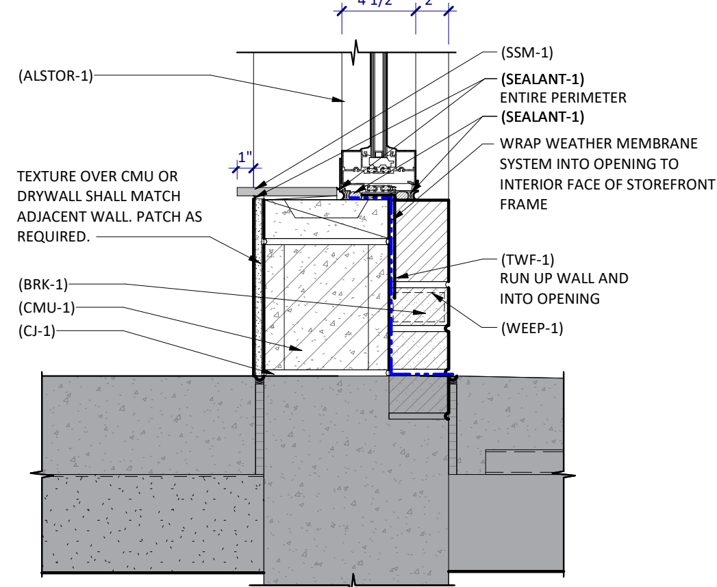
3A A311 ENTRY BRICK SILL DETAIL SCALE: 1 1/2" = 1'-0"
