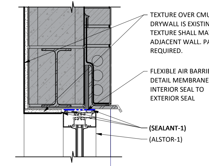
6A A311 EXISTING BRICK HEAD DETAIL SCALE: 1 1/2" = 1'-0"
