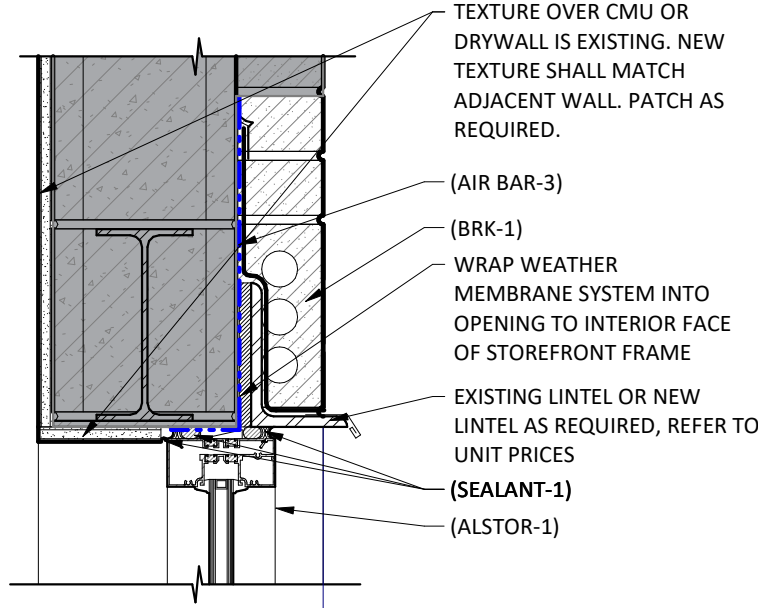
4A A311 BRICK HEAD DETAIL SCALE: 1 1/2" = 1'-0"
